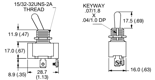
15 & 20 Amp Toggle Switch
