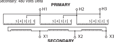
T600L Wiring Diagram & Connections*
