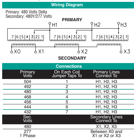
T480J Wiring Diagram & Connections*
