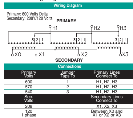
T600A Wiring Diagram & Connections*
