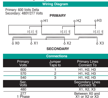
T600H Wiring Diagram & Connections*
