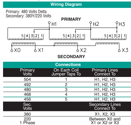
T480K Wiring Diagram & Connections*
