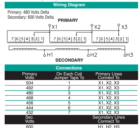
T480T Wiring Diagram & Connections*
