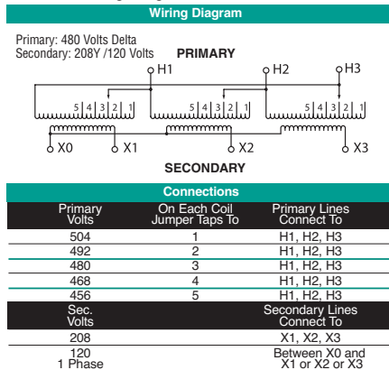
T480M Wiring Diagram & Connections*
