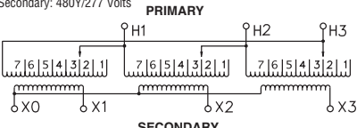
T600M Wiring Diagram & Connections*
