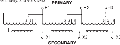
T600J Wiring Diagram & Connections*
