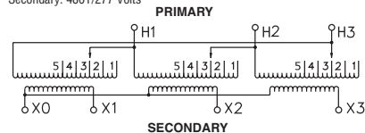
T600I Wiring Diagram & Connections*
