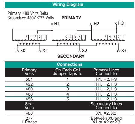
T480P Wiring Diagram & Connections*
