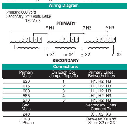
T600F Wiring Diagram & Connections*
