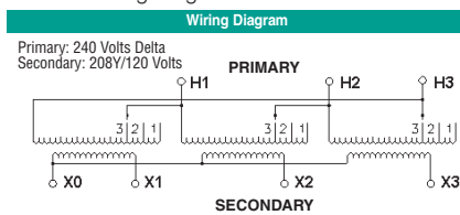
T240A Wiring Diagram & Connections*
