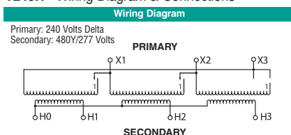
T240H Wiring Diagram & Connections*
