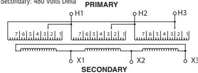
T600K Wiring Diagram & Connections*
