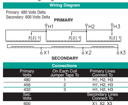
T480R Wiring Diagram & Connections*
