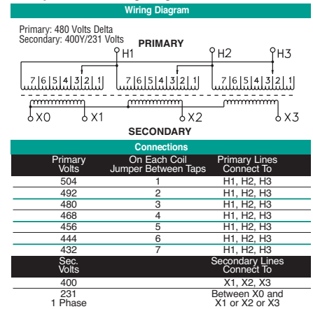
Group T480L Wiring Diagram & Connections*
