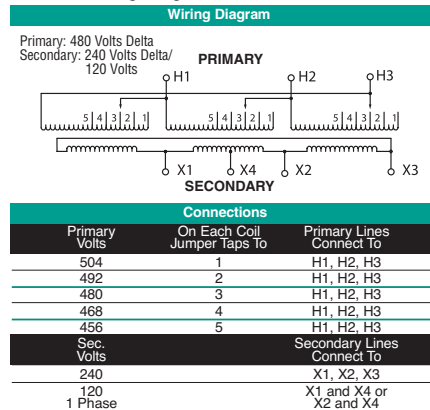
T480N Wiring Diagram & Connections*
