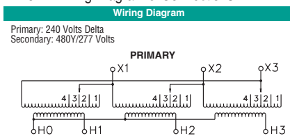
T240E Wiring Diagram & Connections*
