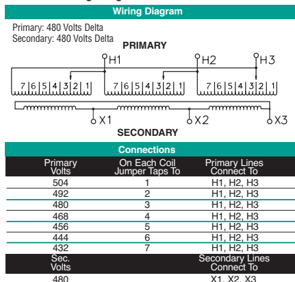
T480Q Wiring Diagram & Connections*
