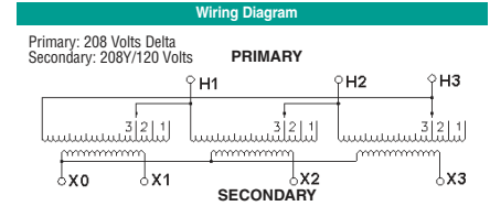
T208H Wiring Diagram & Connections*
