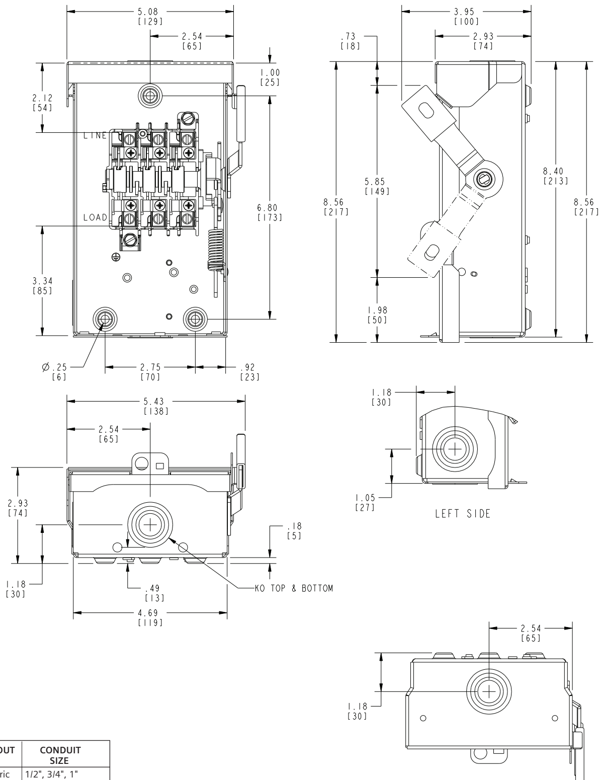
Type 1 (Indoor) 60 Amp Non-fusible
