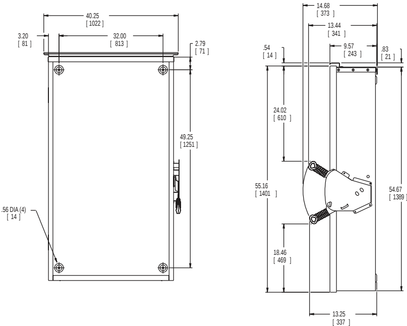
800 / 1200 Amp Heavy Duty Fusible
