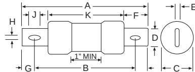
Class J Blade type 61-600A
