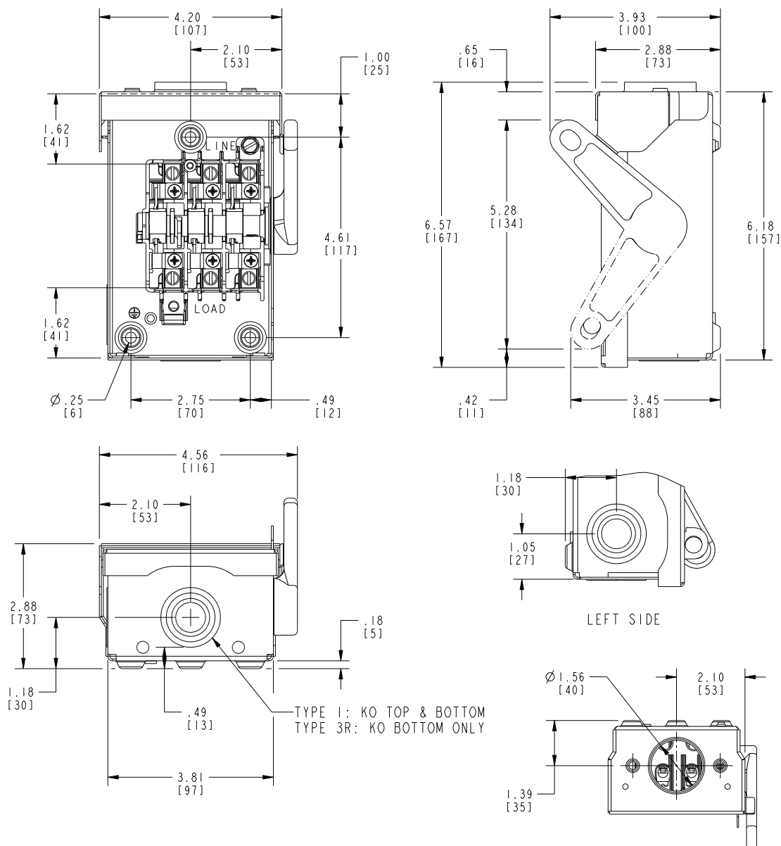
Type 3R (outdoor) 30 Amp Non-fusible
