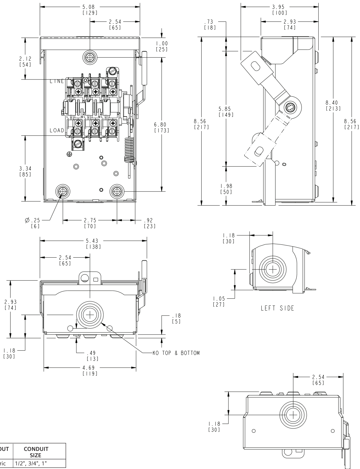
Type 1 (Indoor) 30 Amp Oversize Non-fusible
