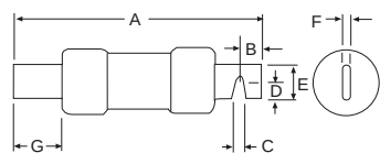
Blade type 61-600A
