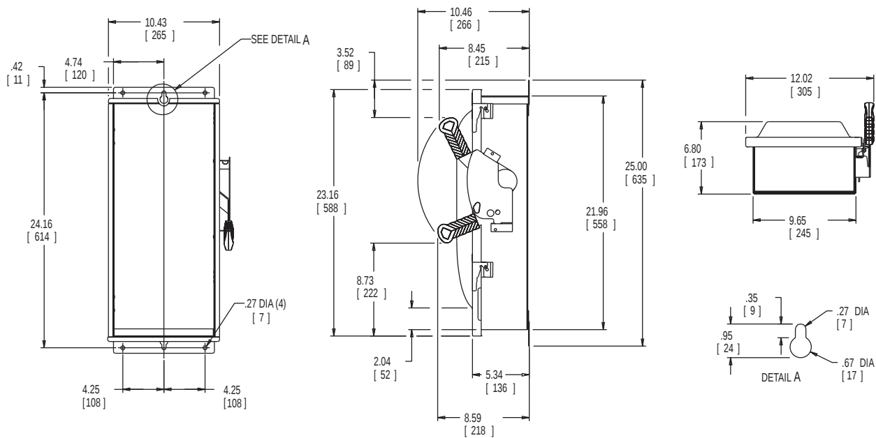
100 Amp Heavy Duty
