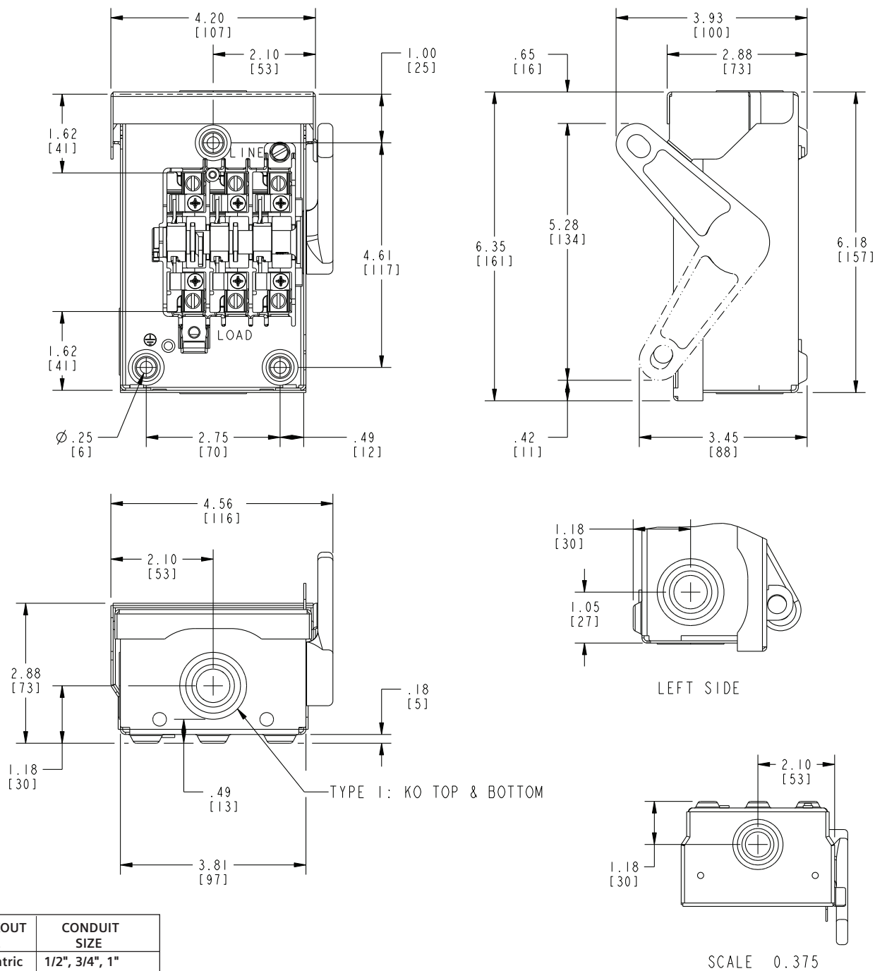
Type 1 (Indoor) 30 Amp Non-fusible
