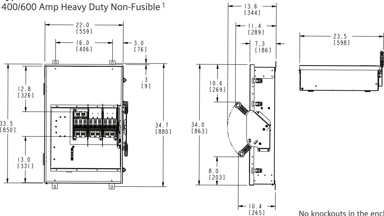
Type 12 (Industrial) 400/600 Amp Heavy Duty Non-Fusible 1
